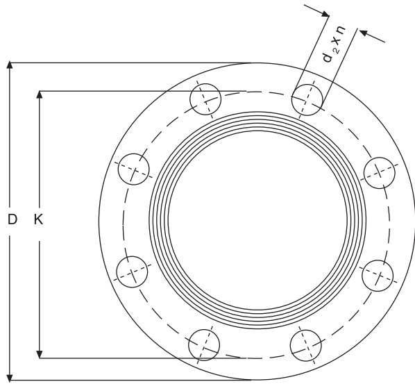
KÖR FLANŞ 300 LB BLIND FLANGE CLASS 300 (ASME B 16.5 - 1996 + MSS - SP 44 - 1996) B16.47 - A / B16.47 - B
